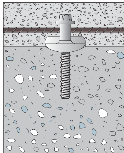
Connector supplied with toothed plate and screw with threaded body, length 65 mm.
